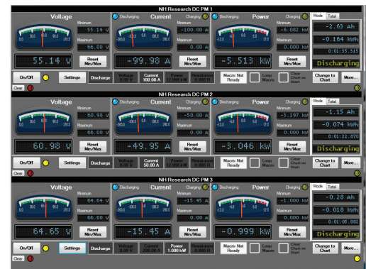
Three Channel Monitor Panel
