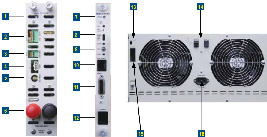
Fig. 6 - Front panel (300W load) & Front panel control
