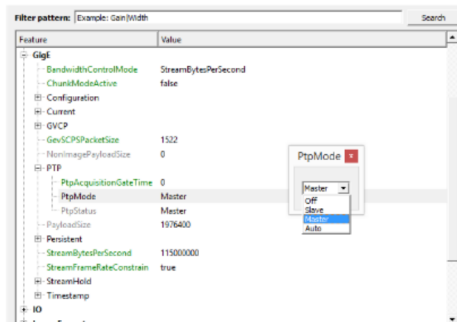
Figure 3: PtpMode in Vimba Viewer
