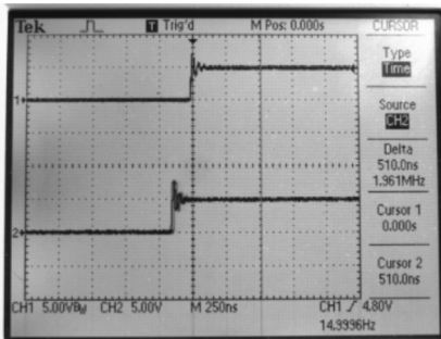
Figure 7: Scope image of oscilloscope showing trigger waveforms
