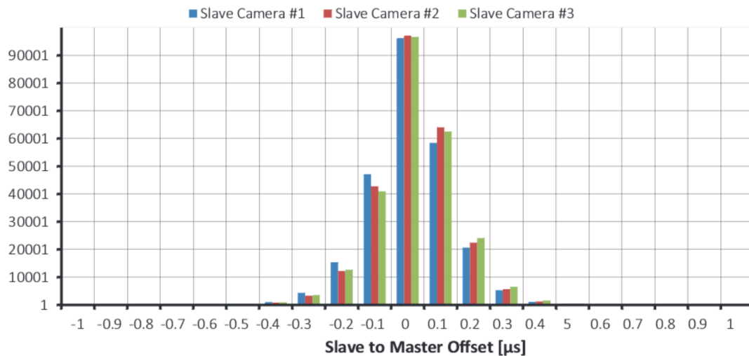
Figure 6: Histogram of slave to master offset
