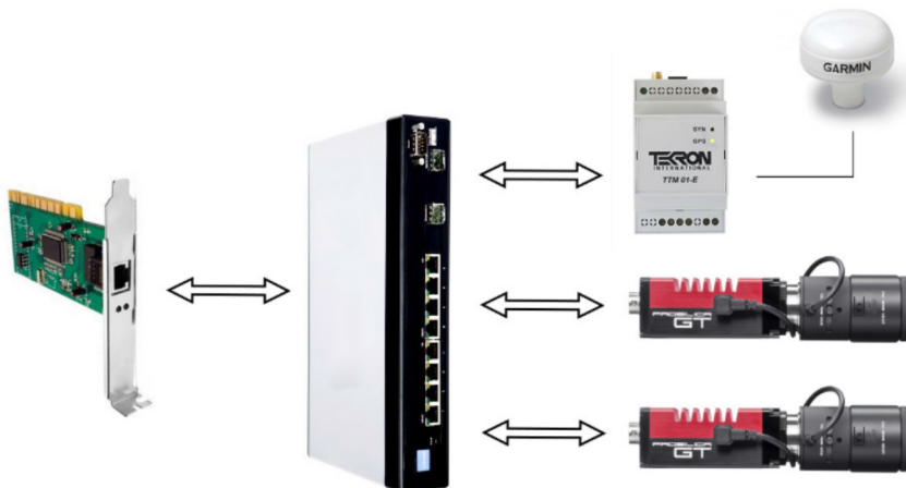
Figure 5: Synchronization using GPS clock
