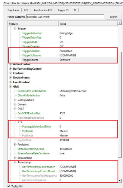
Figure 4: PTP features in the Vimba Viewer
