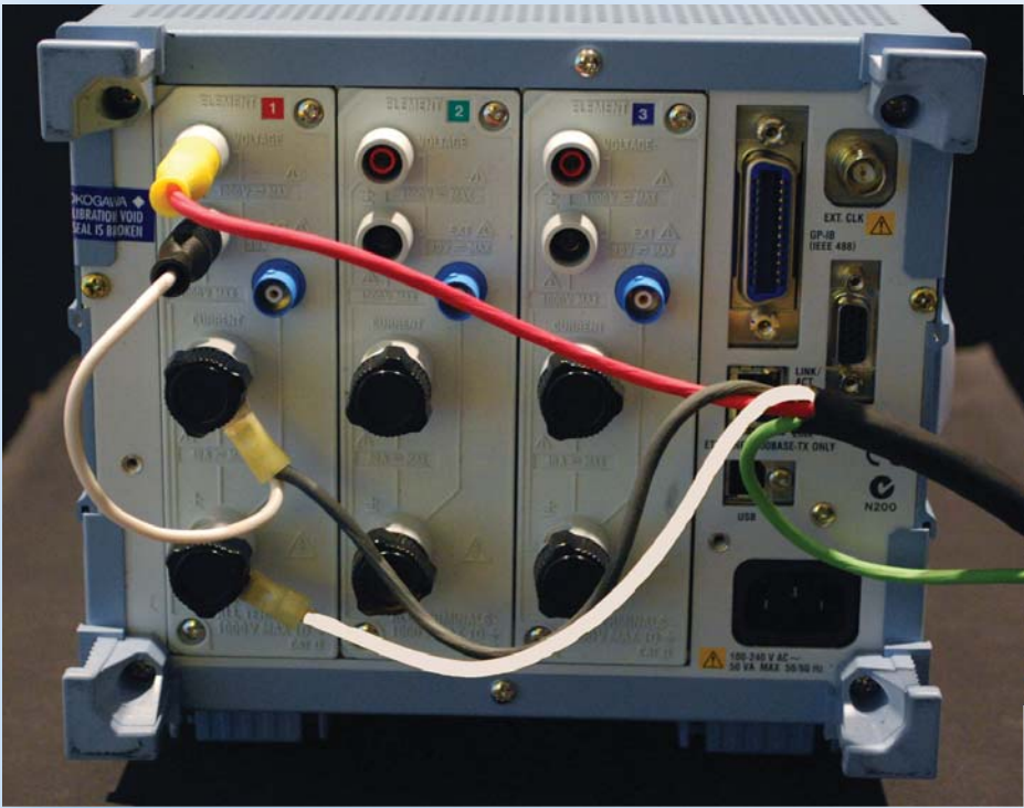
neoXT - WT500 Connections
