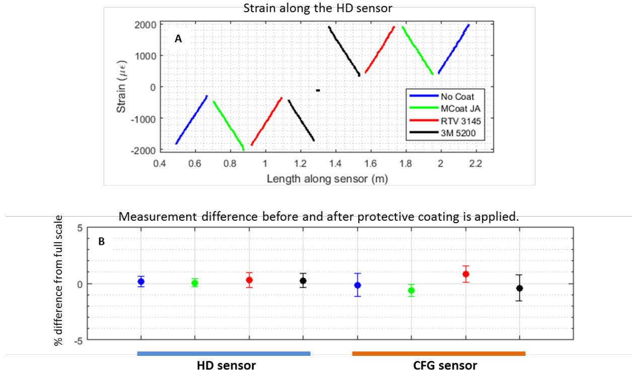
Figure 2: A. Strain distribution along the length of a HD sensor. B. Measurement difference before and after a protective coating is applied.
