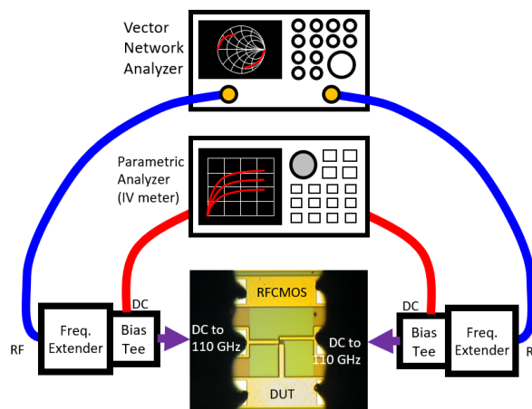
Fig.1 Schematic with die photo showing a typical wafer-level setup to test RF transistor up to 110 GHz.
