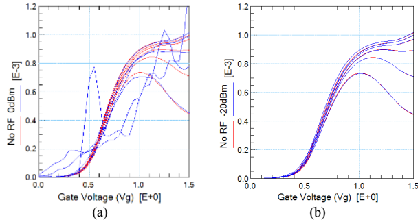
Fig. 2. DC transconductance versus gate voltage ( G_m vs v_g ) at different drain voltages at 0.3, 0.6, 0.9, 1.2, 1.5 and 1.8V, for a RF nMOSFET with network analyser RF power OFF "HOLD" (Red plot) comparing with RF source power = 0 dBm (a) and RF source power = -20 dBm (b) (Blue plots).
