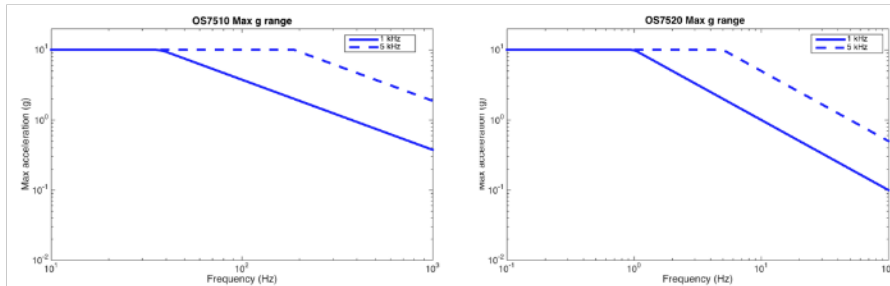
Shown is the actual peak acceleration that can be measured on the os7510 (left) and os7520 (right) as a function of the frequency of the applied acceleration when measured with a HYPERION si155/255 instrument operating with a 1 kHz and 5 kHz scan rate.
