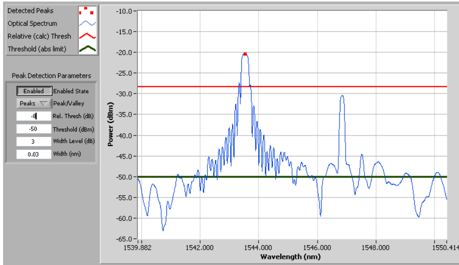
Case E: Insertion loss on a single FBG loss leads to a missing peak
