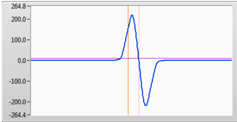
Differential Delay, where the zero crossing serves as an indicator of the peak location.
