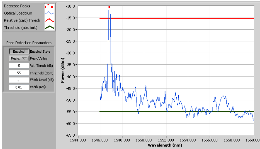
Case I: Single FBG, Rel. Thresh sets effective threshold far above noise floor.
