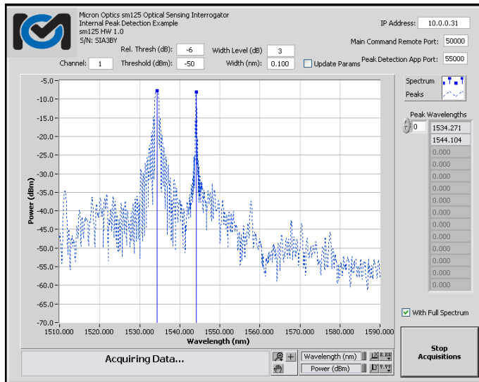
sm125 Internal Peak Detection Example
