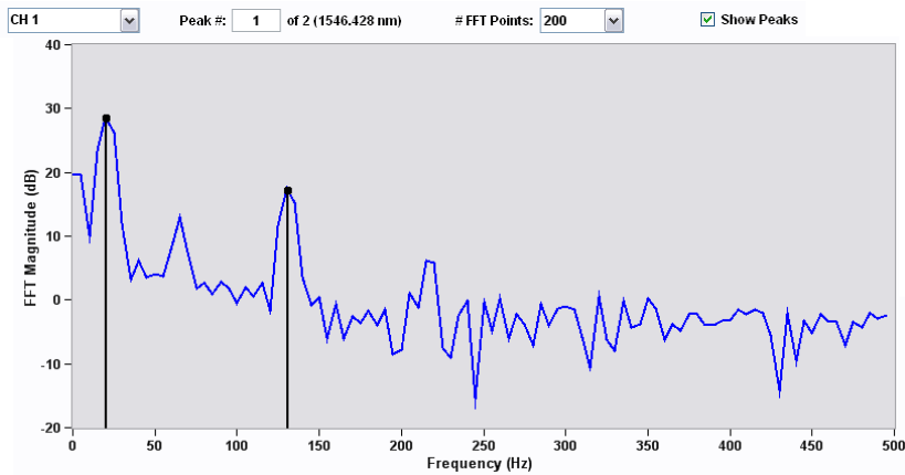
Spectral Peak FFT view
