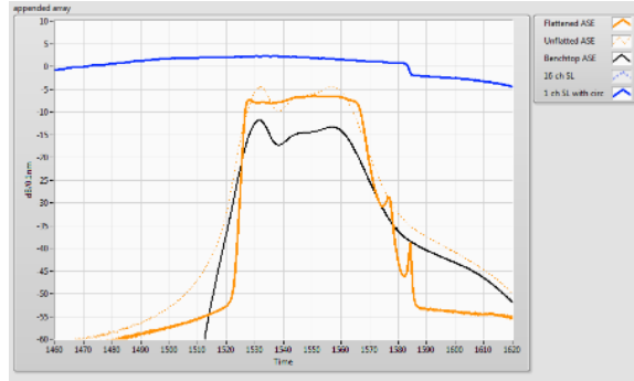
The figure above shows the high output power and wide wavelength range of the si255 swept wavelength laser (blue) in comparison to traditional Erbium ASE sources (orange and black).
