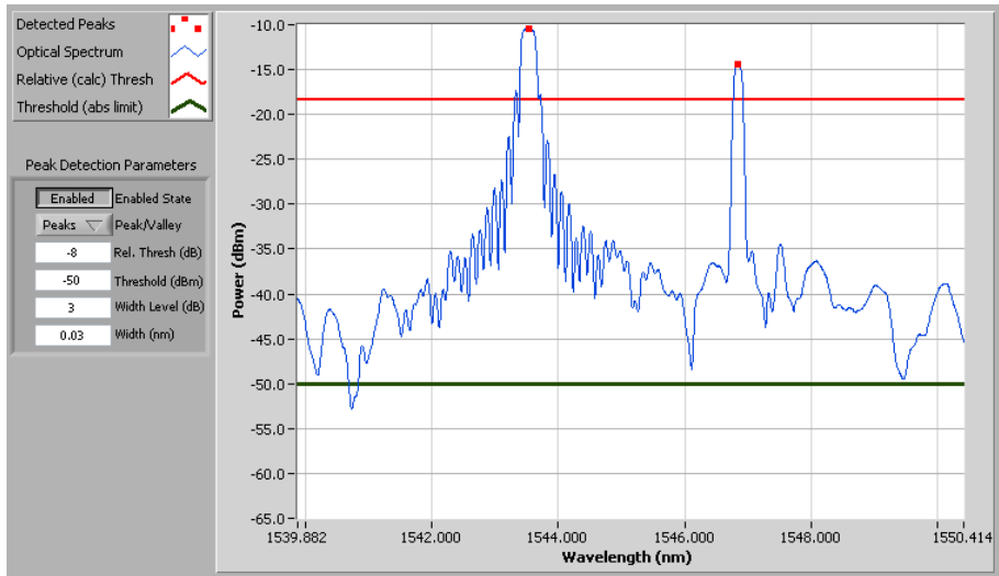
Case C: Relative thresholding used with a low-loss signal.
