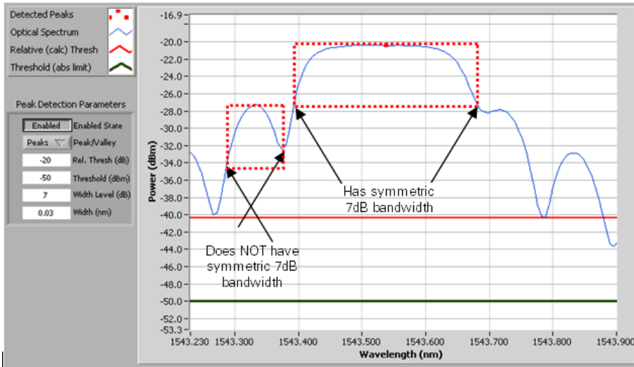
Case H(2). The fundamental mode has a symmetric 7 dB bandwidth, but the side lobe does not.
