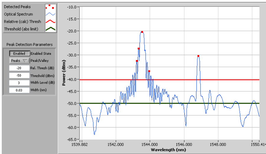
Case F: Reduction of the Rel. Thresh parameter allows for FBG 2 detection, but also includes several side modes from FBG 1.
