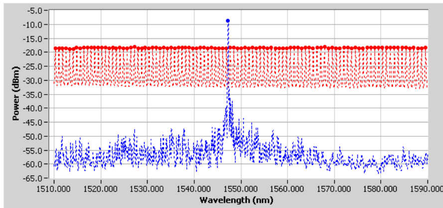
x25 full spectrum trace with peak detection results
