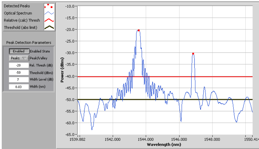
Case H(1). Keep original PD width parameter, but change the Width Level to take advantage of spectral symmetry of fundamental FBG modes
