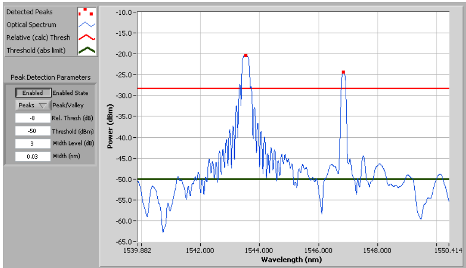
Case D: Use of relative thresholding allows for changes in insertion loss without the need to change peak detection parameters.
