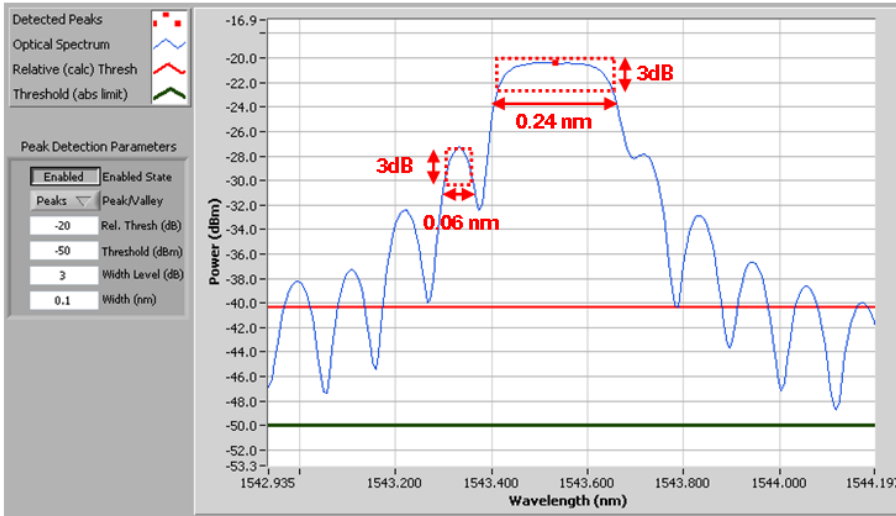
Case G(2). A close up reveals that the 3 dB bandwidth of the fundamental mode is greater than the required 0.1 nm, while the 3dB bandwidth of the side mode is not.
