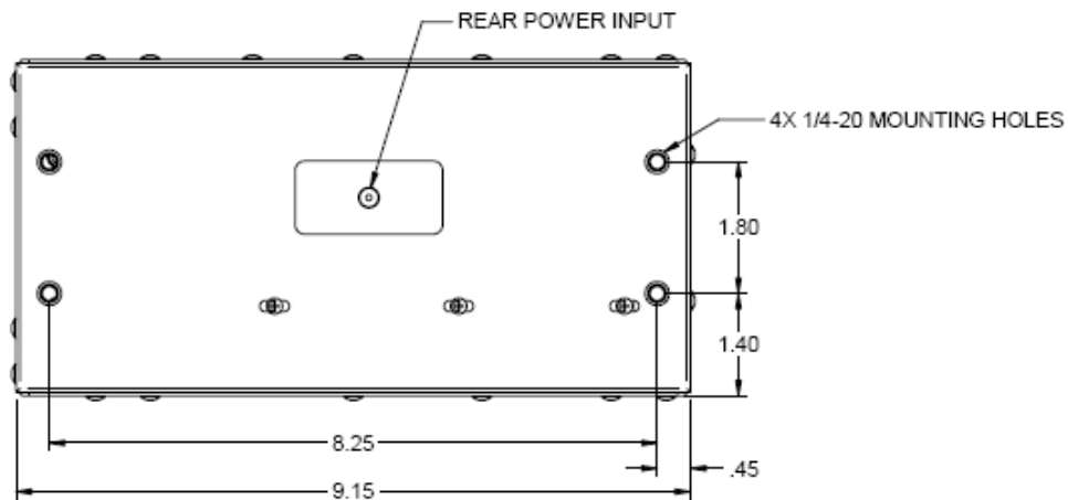
sm125-500 Rear View
