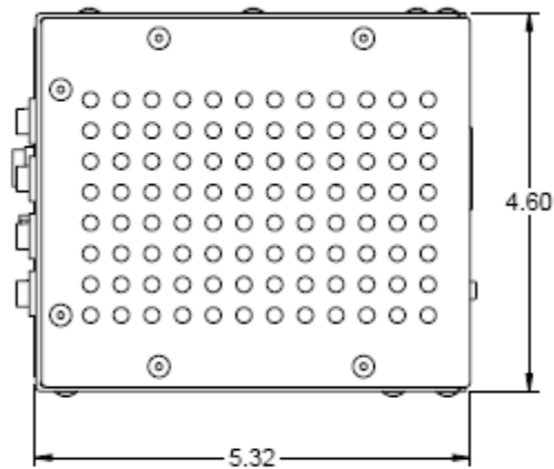
sm125-500 Side View
