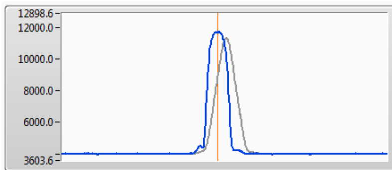
“Raw” signal, not scaled for power calibration (blue). Low pass “Box Car Filter” output of the first DSP block (gray).
