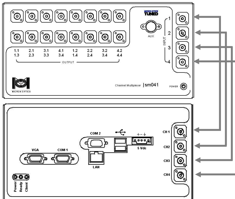
Diagram of sm041 optically connected to host instrument.
